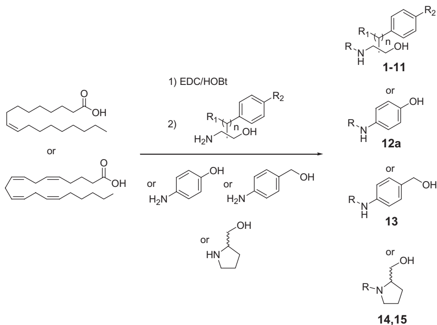
Figure 2. Synthesis of compounds 1–15.
